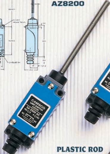
COIL SPRING ROD AZ8200
