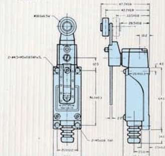
ADJUSTABLE LENGTH ROLLER LEVER AZ8108
