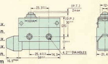
Compact overtravel plunger
