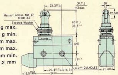
Panel mount roller plunger
