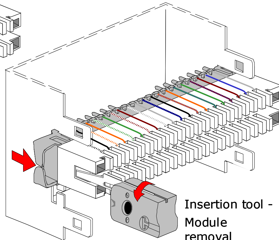
Removing module
