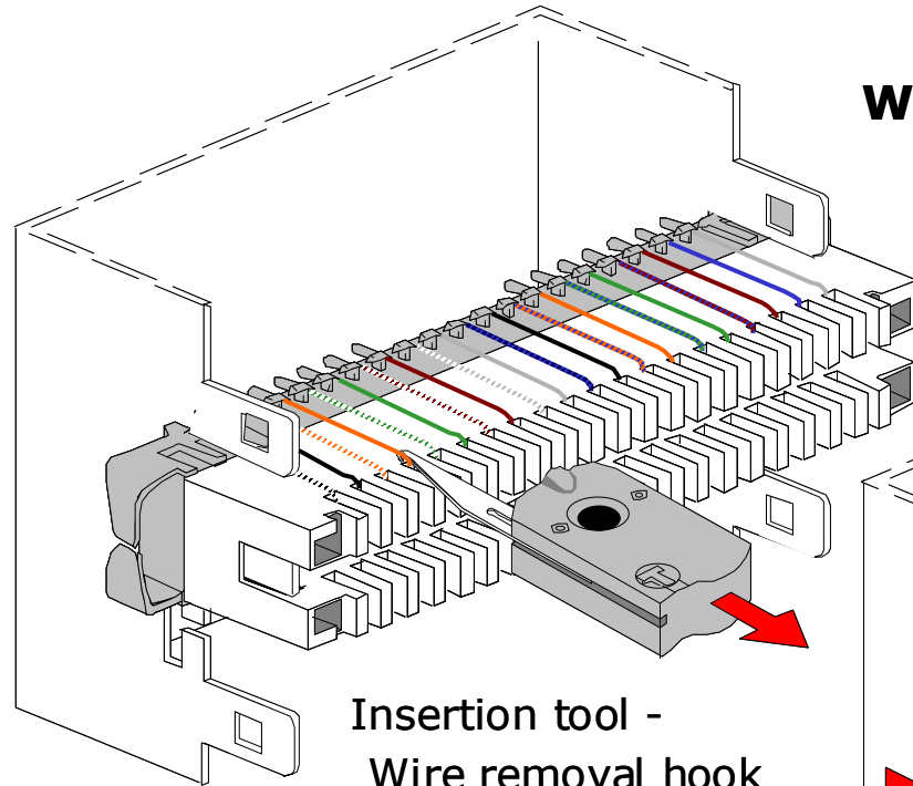
Removing wiring
